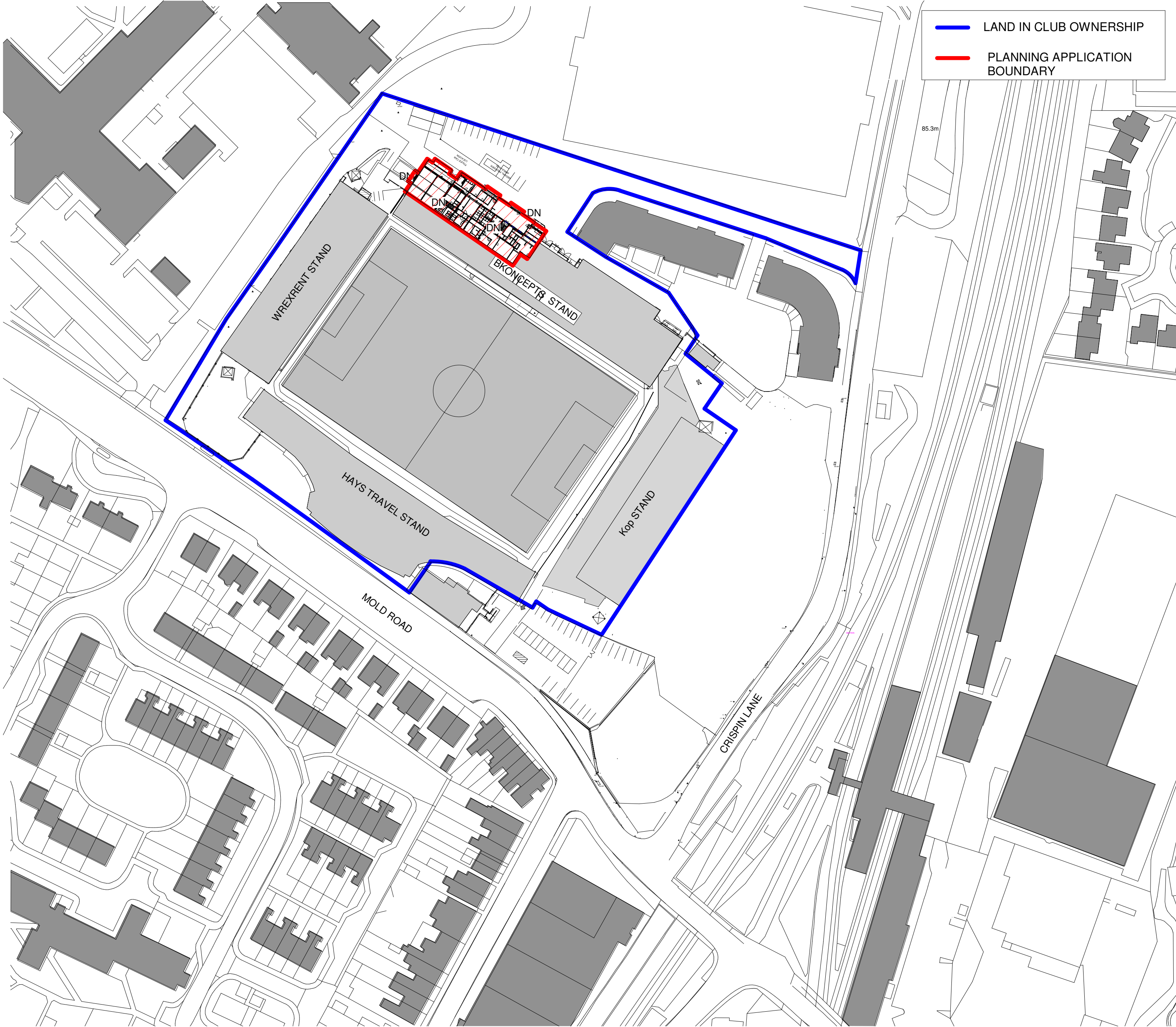
1 Site Location Plan 1 : 1000
