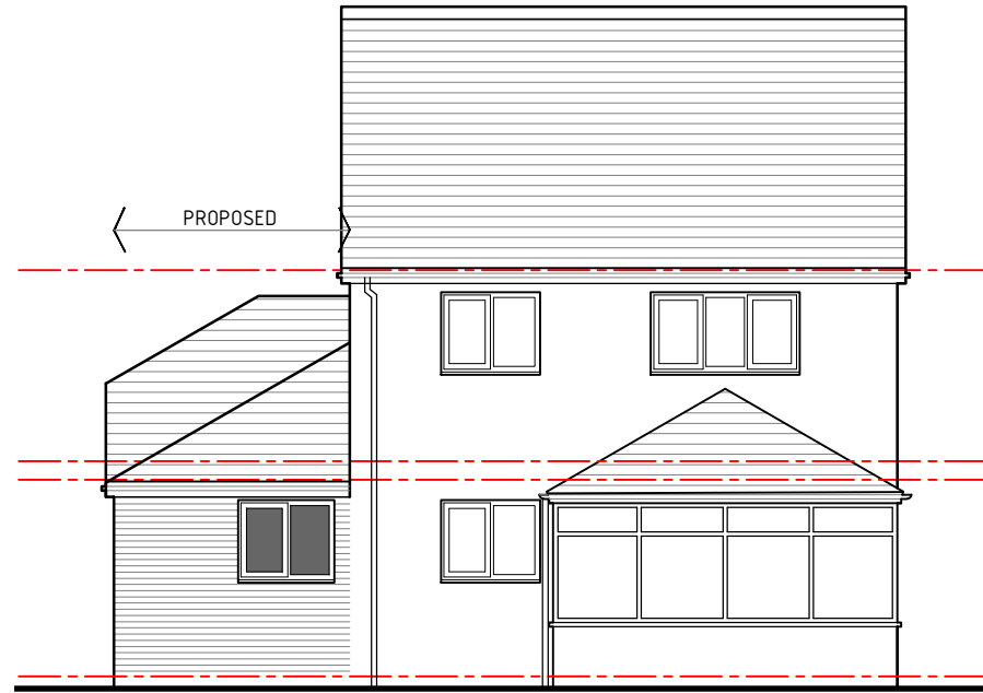
Rear Elevation 1:100
