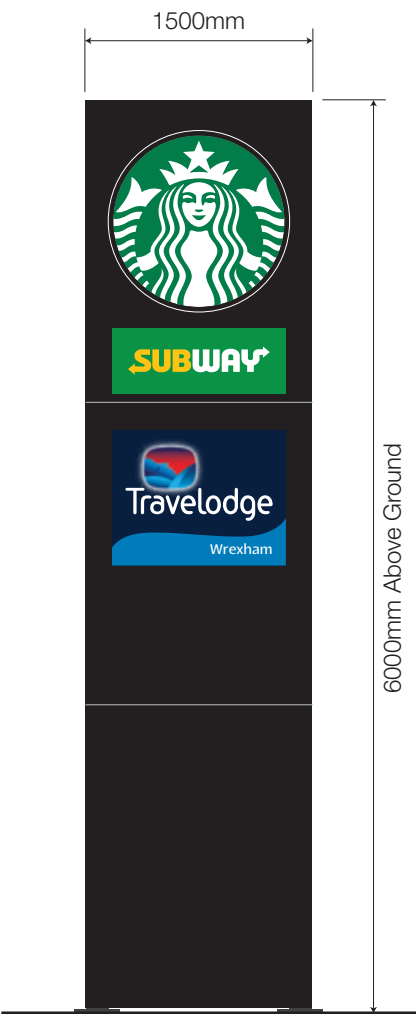
Rear Elevation - 1:50
