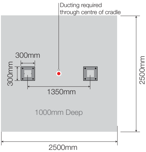
Groundworks - 1:50
