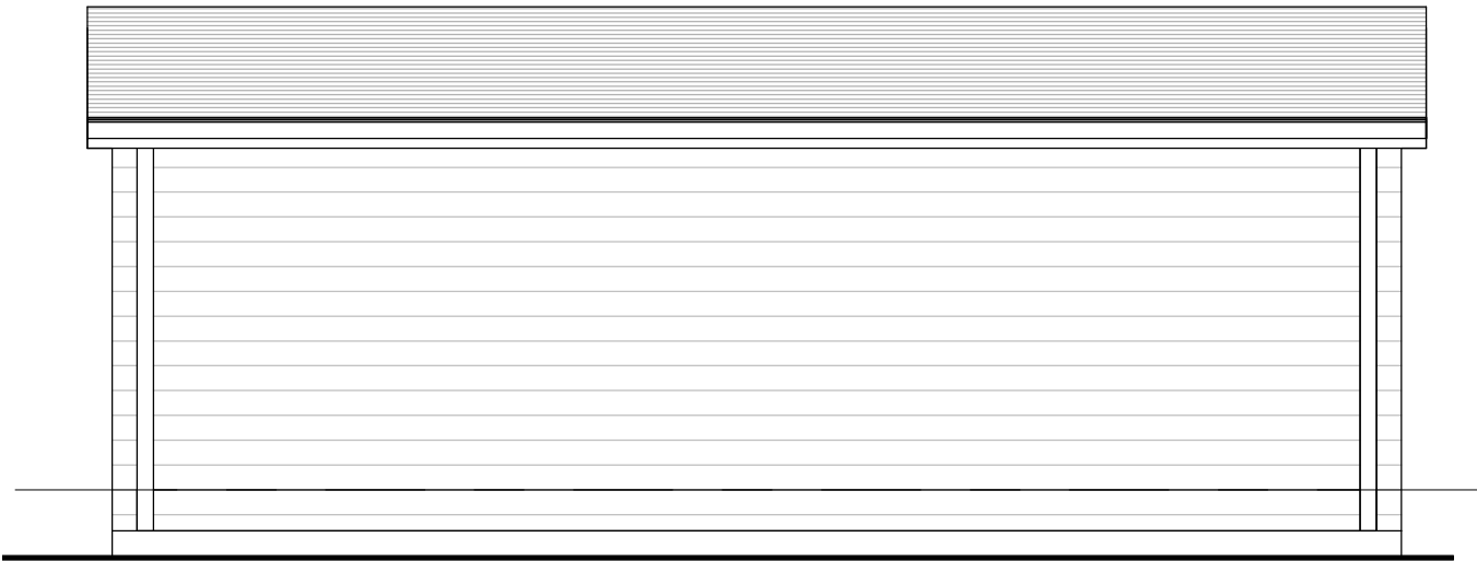
East Elevation 1 : 50
