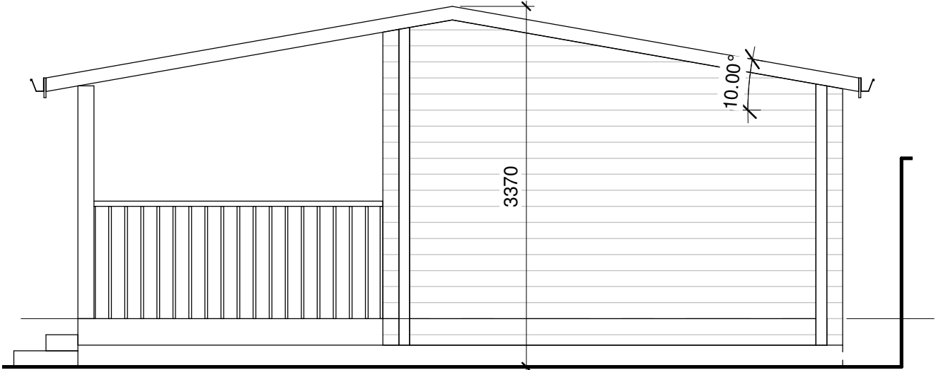
North Elevation 1 : 50
