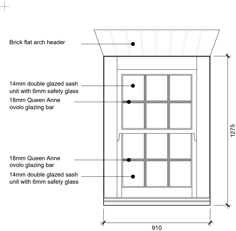
PROPOSED WINDOW ELEVATION
