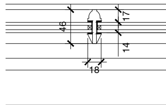
PROPOSED GLAZING BAR DETAIL (1:5)
