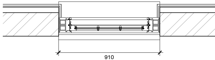
PROPOSED WINDOW PLAN
