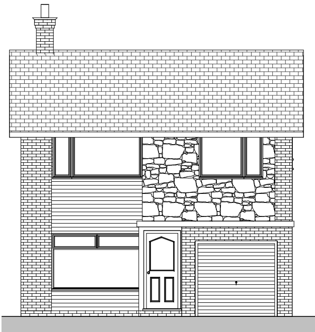
Front Elevation 1 : 100
