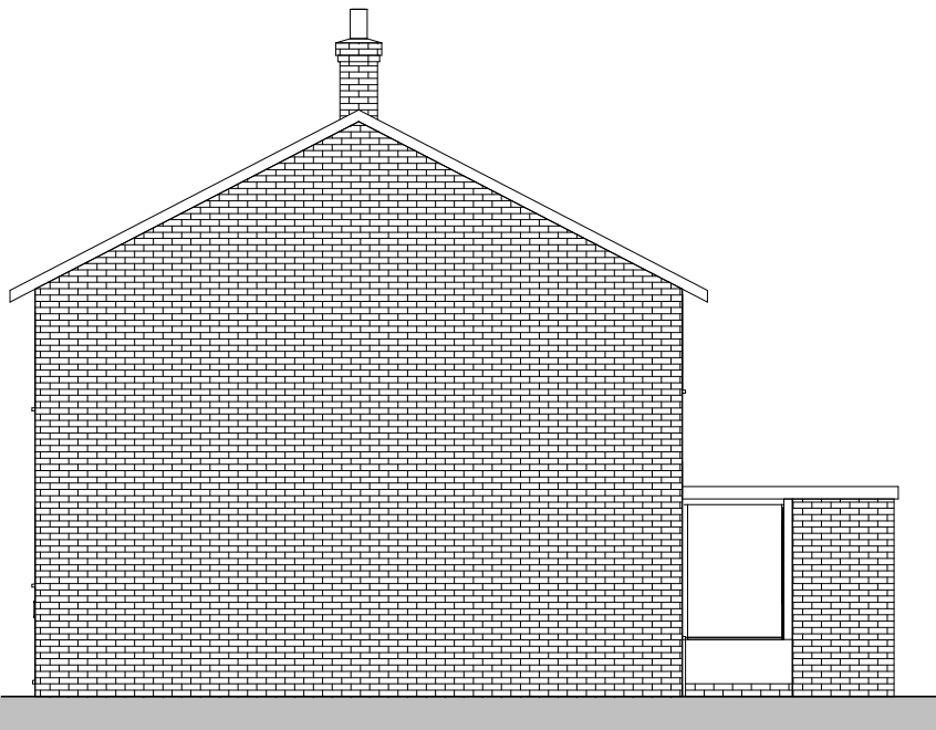
Side Elevation 1 : 100
