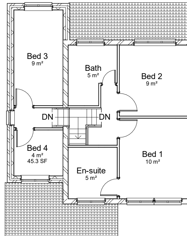
2 Proposed First Floor Plan 1 : 100
