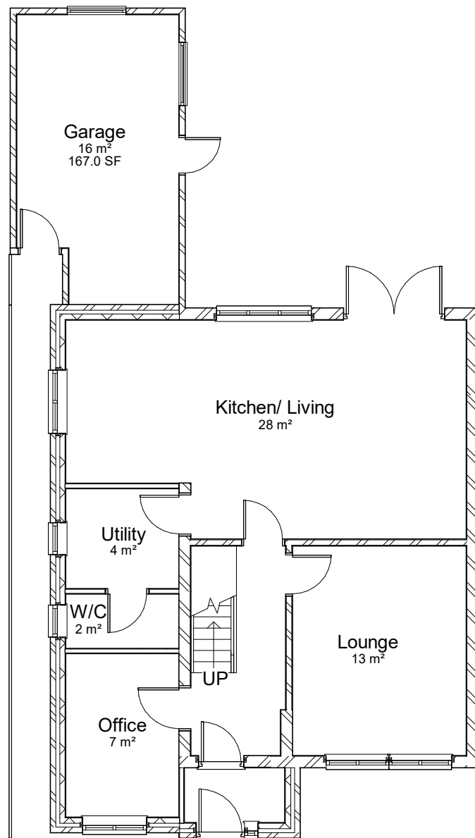
1 Proposed Ground Floor Plan 1 : 100
