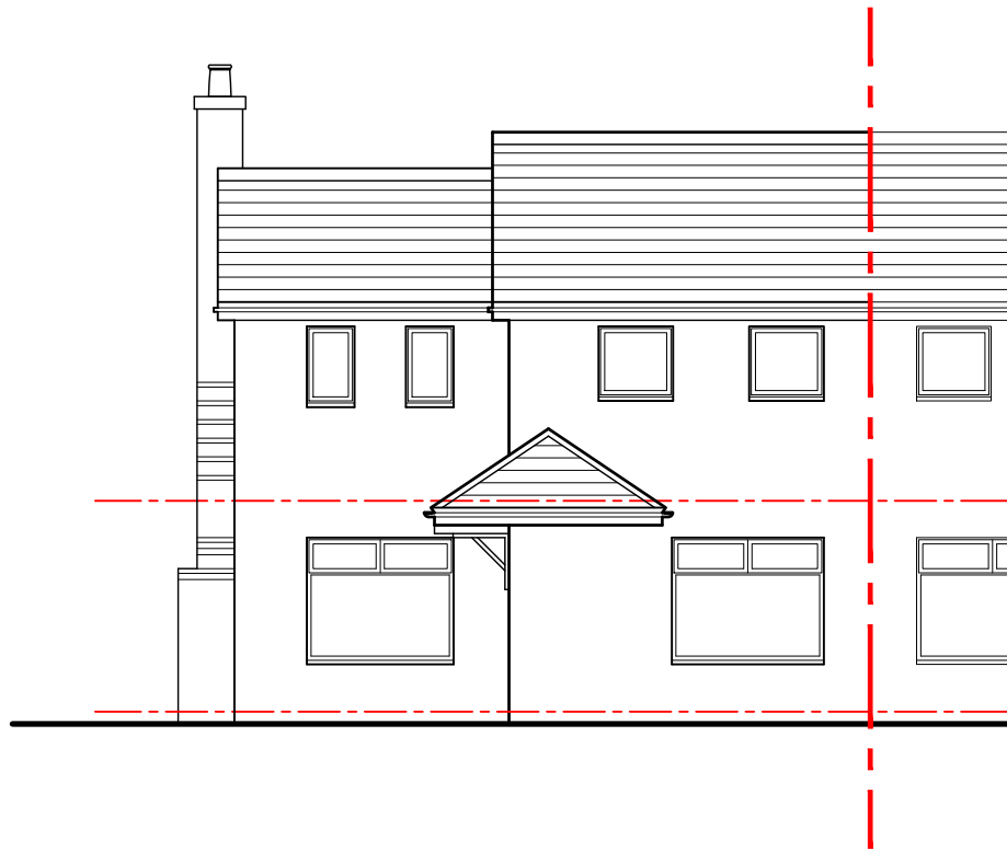
Front elevation 1:100
