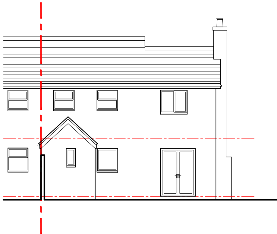
Rear elevation 1:100
