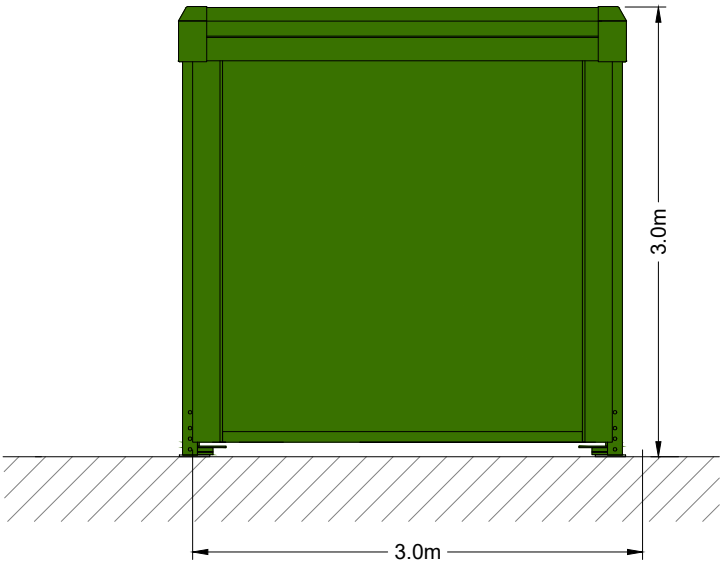
NORTHERN ELEVATION
