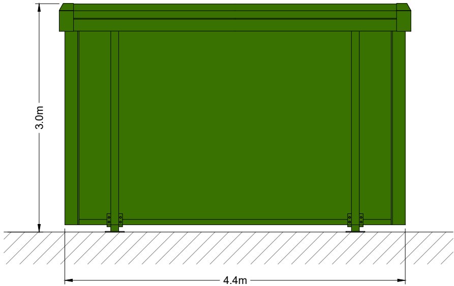
WESTERN ELEVATION
