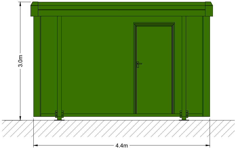
EASTERN ELEVATION
