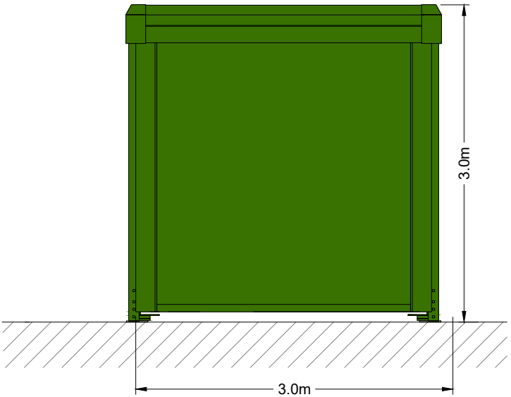
SOUTHERN ELEVATION
