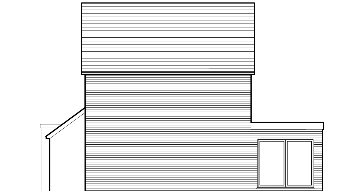
2 SIDE ELEVATION
