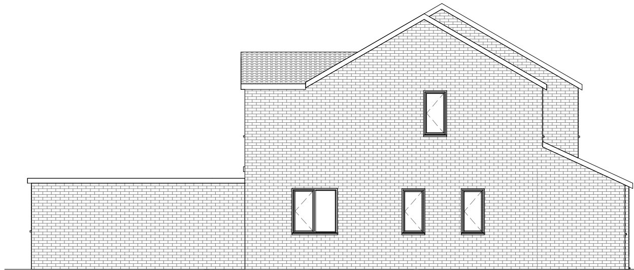
2 Proposed East 1 : 100
