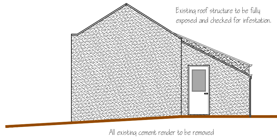
EXISTING GABLE 1 ELEVATION SCALE 1:100
