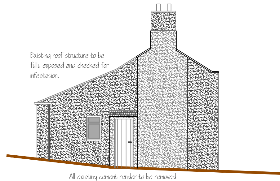
EXISTING GABLE 2 ELEVATION SCALE 1:100
