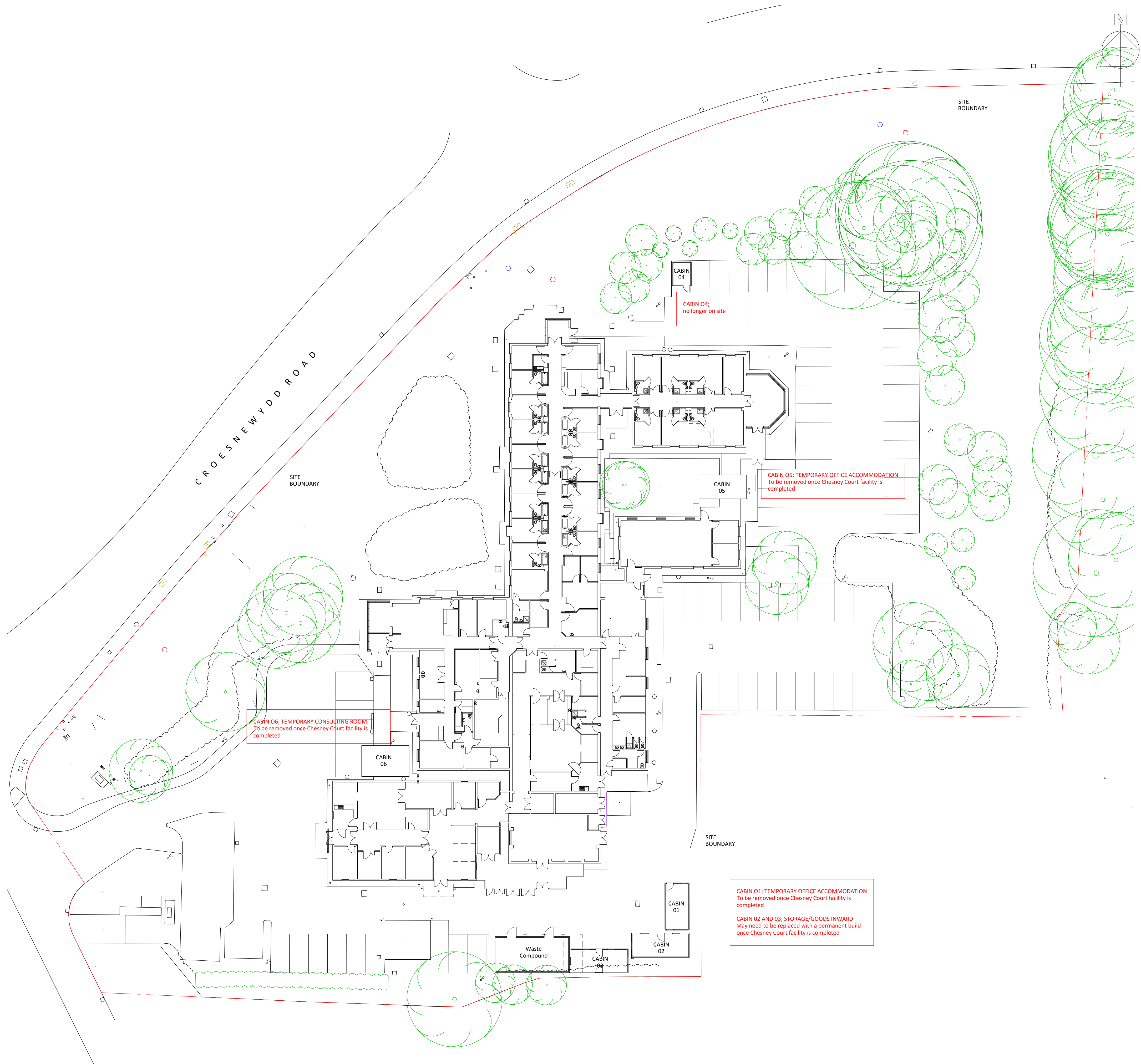
BLOCK PLAN Scale 1:500
