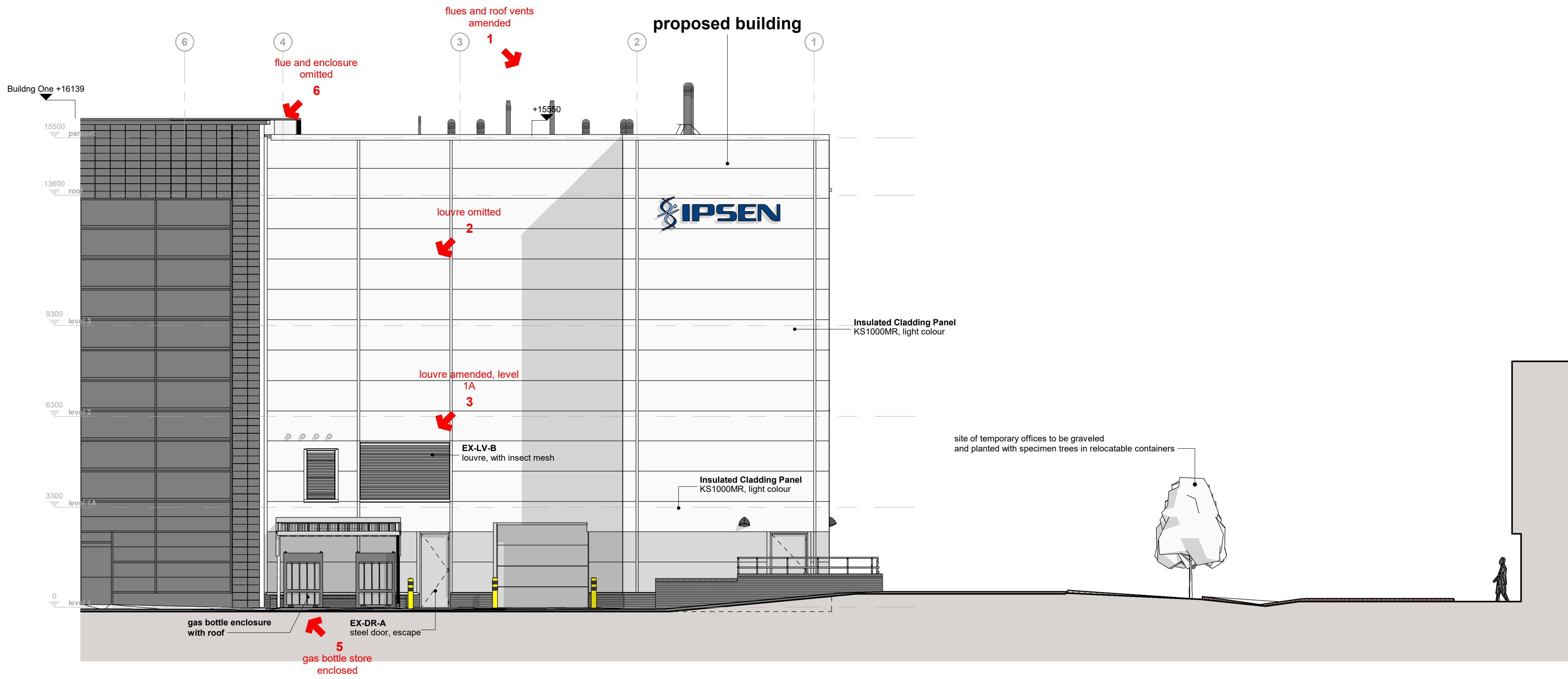
E Planning_Elevation_GA_East Scale: 1 : 100
