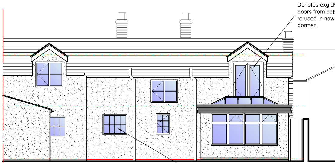
REAR ELEVATION (1:100)
