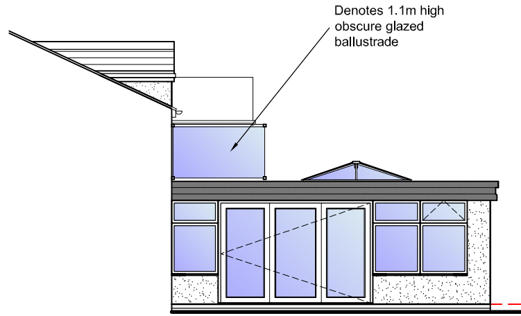
SIDE ELEVATION (1:100)
