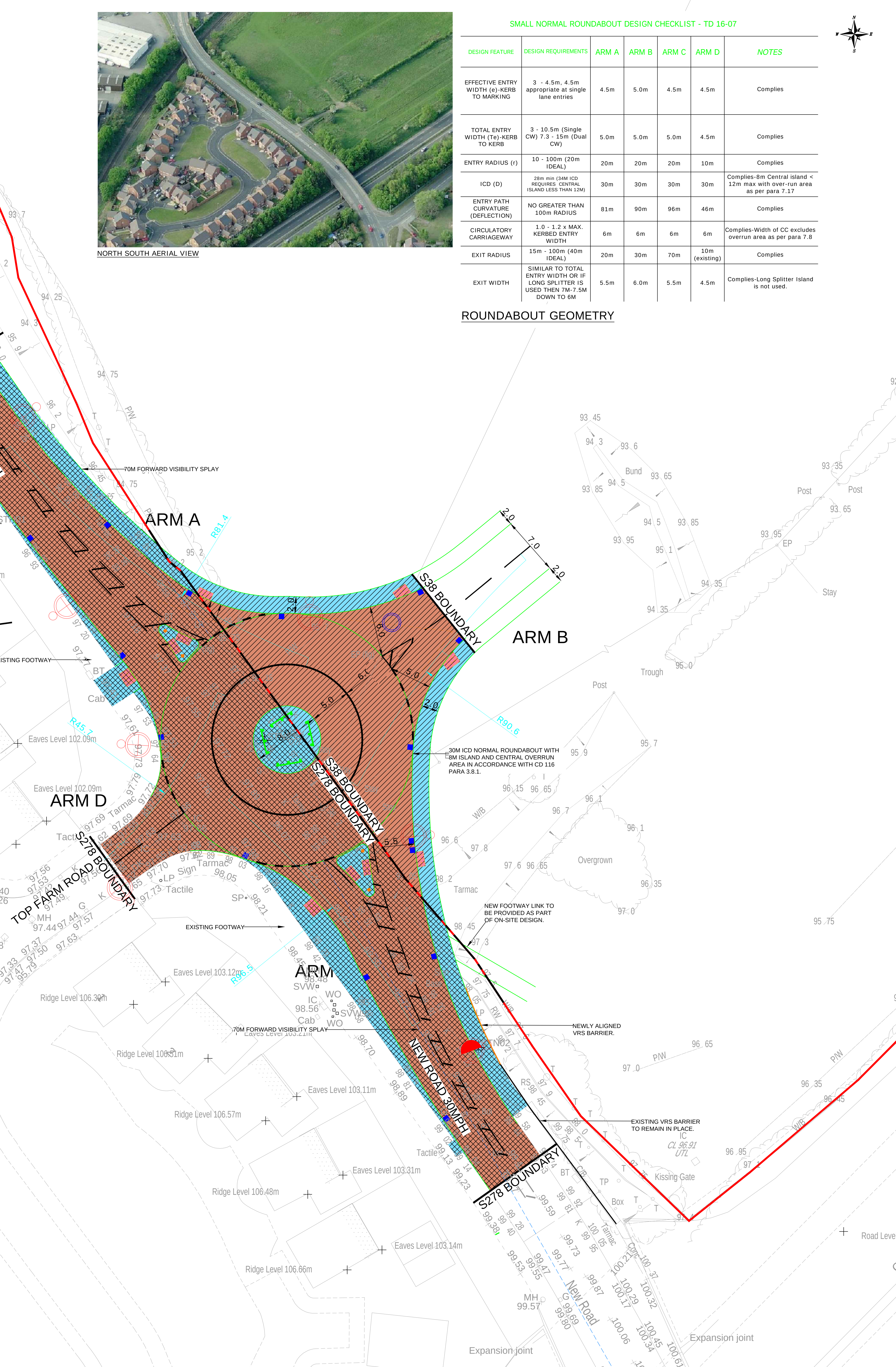
ROUNDABOUT GEOMETRY
