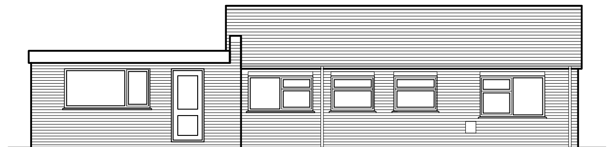
5 REAR ELEVATION
