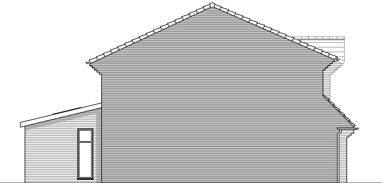
SIDE ELEVATION
