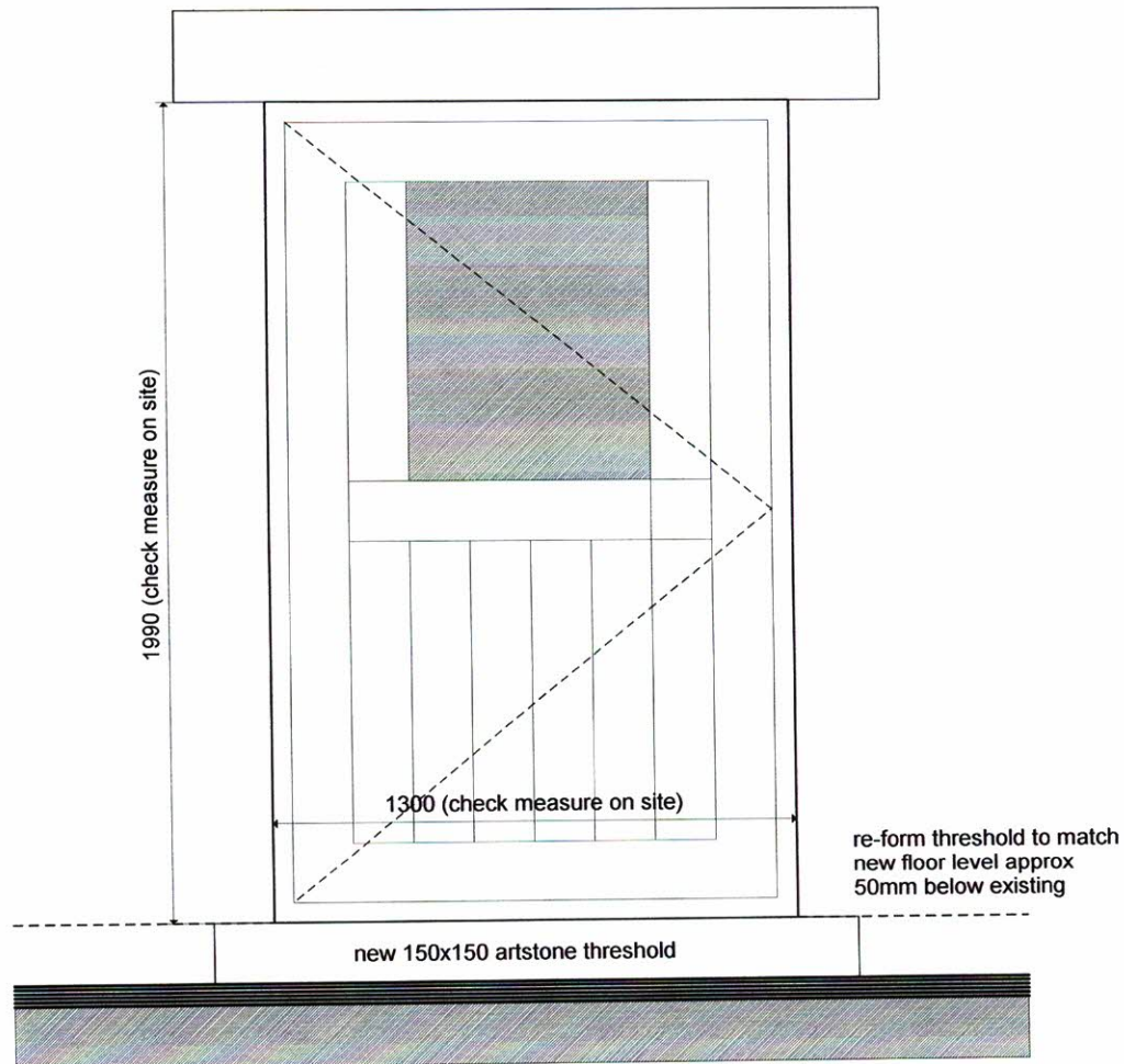
D2 EXTG OPENING 1:20
