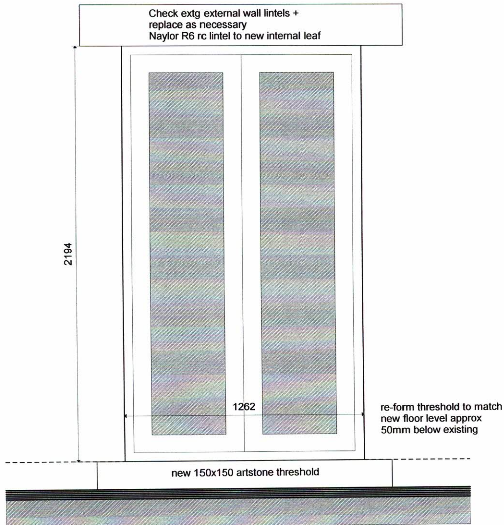
D5 EXTG OPENING REINSTATED TO THRESHOLD LEVEL 1:20
