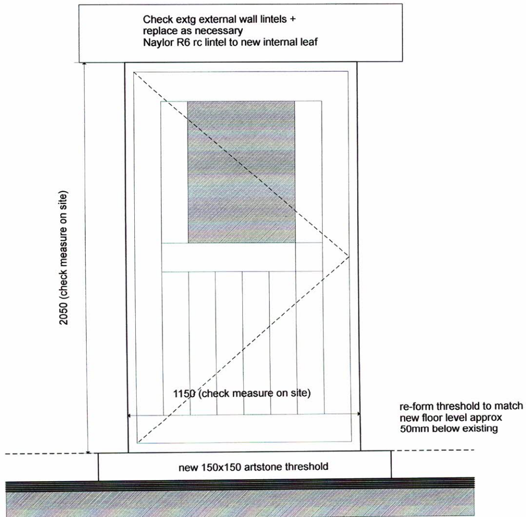
D1 EXTG OPENING 1:20
