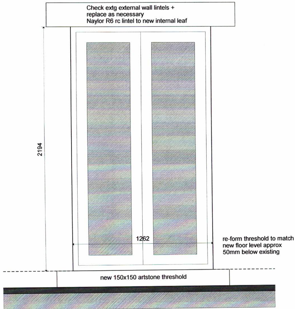
D4 EXTG OPENING 1:20
