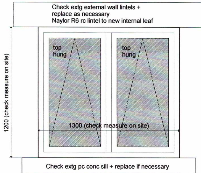
W5 EXTG OPENING 1:20
