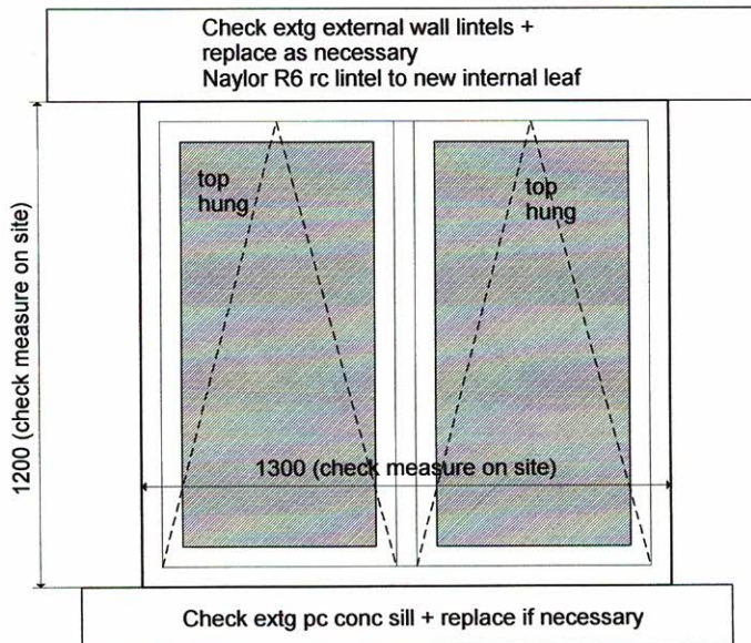
W6 EXTG OPENING 1:20
