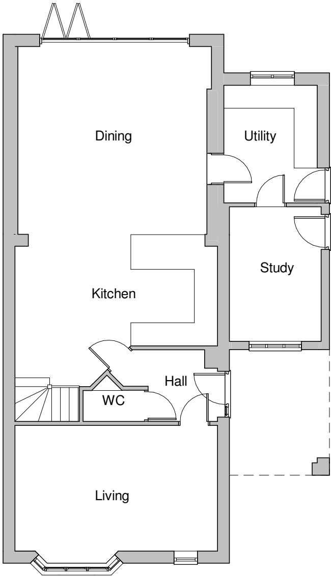
Ground Floor 1 : 100
