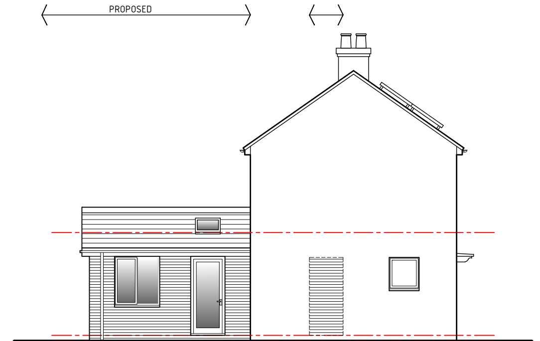
Side-01 Elevation 1:100
