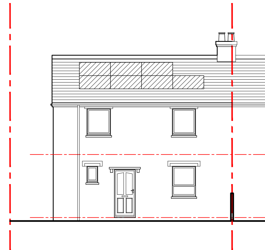
Front Elevation 1:100
