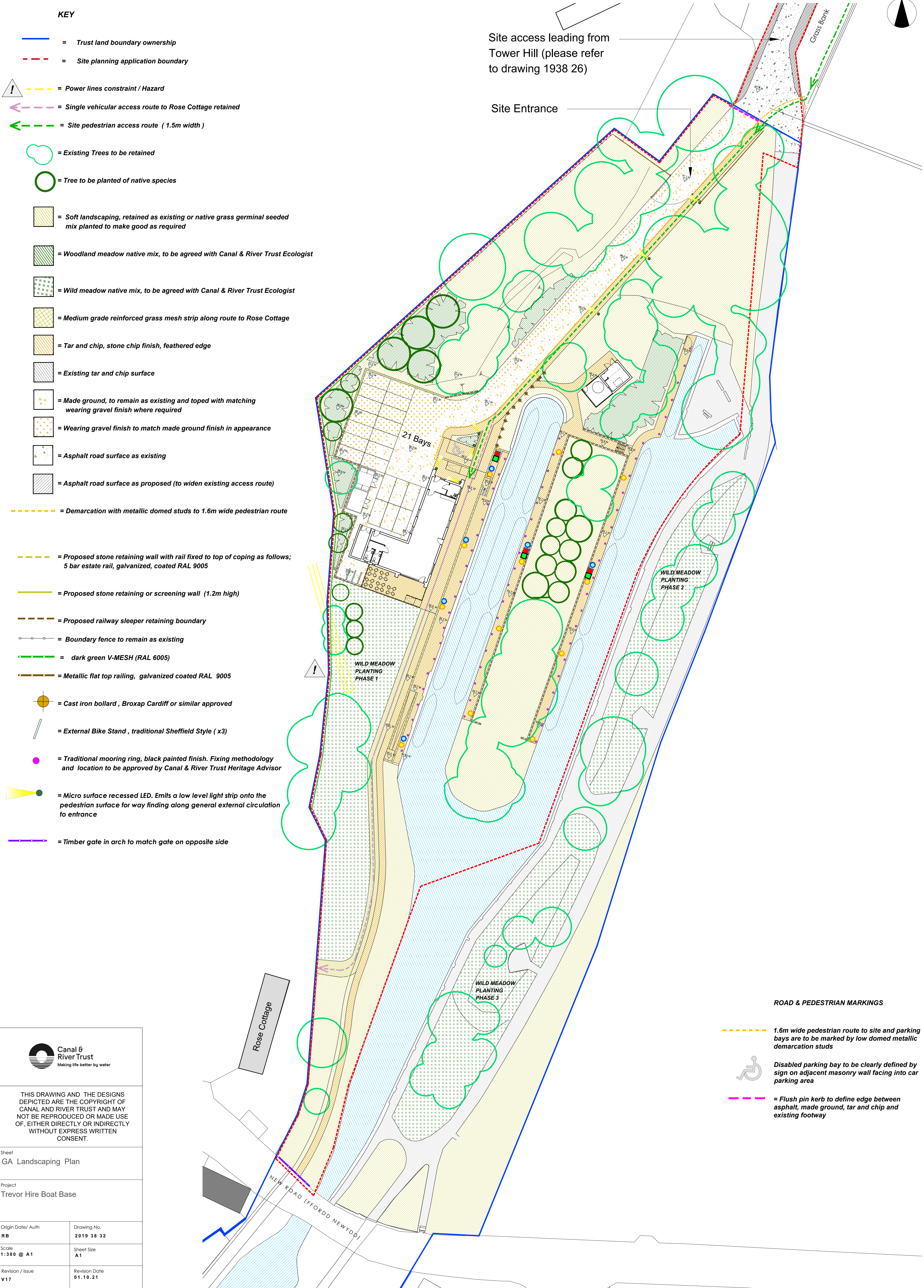
GA LANDSCAPE PLAN Scale 1:300 @ A1
