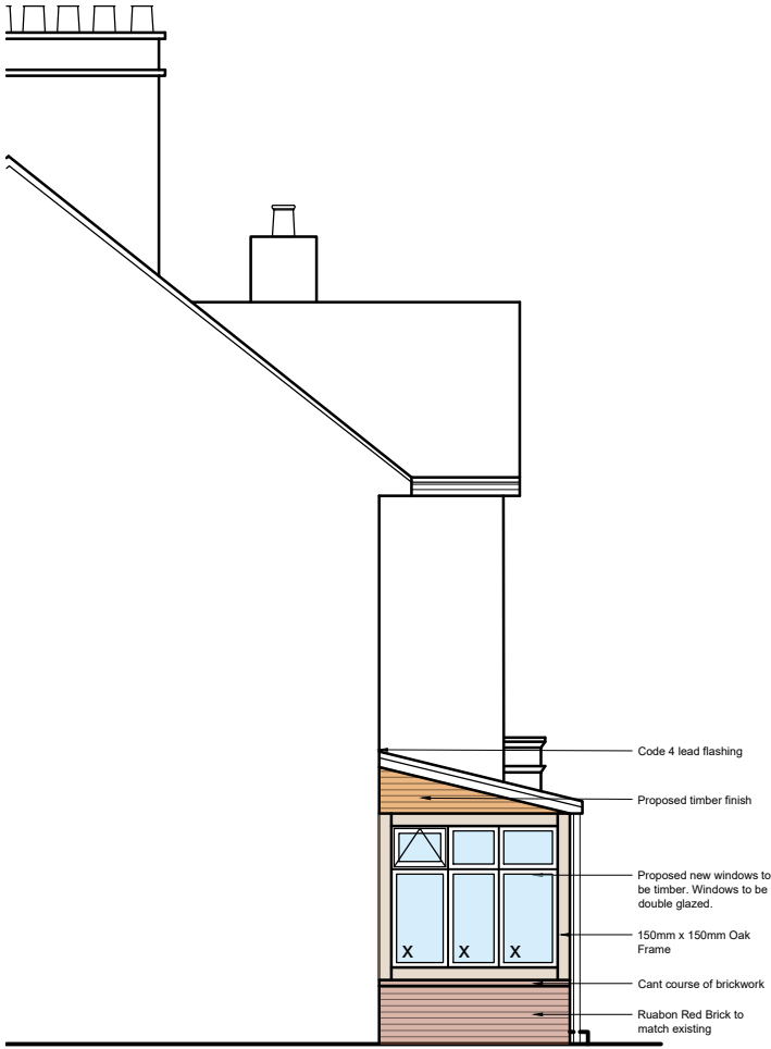
Side 01 Elevation
