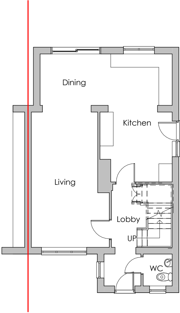
Ground Floor 1 : 100
