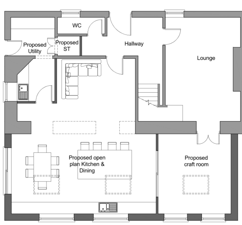
Figure 6 – Proposed Floor Plan
