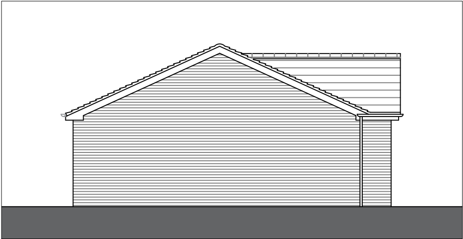
HOUSE SIDE ELEVATION
