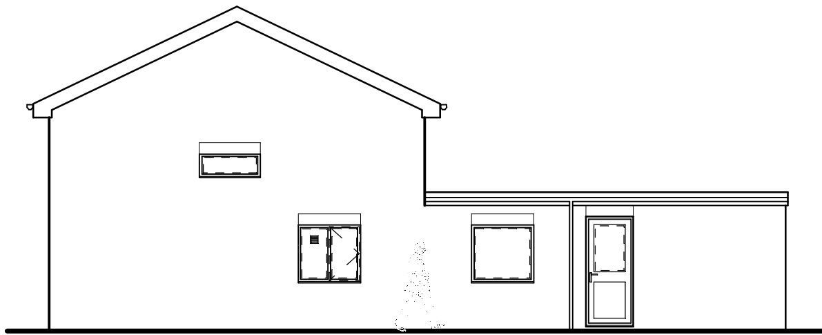
PROPOSED SIDE ELEVATION ( WEST )
