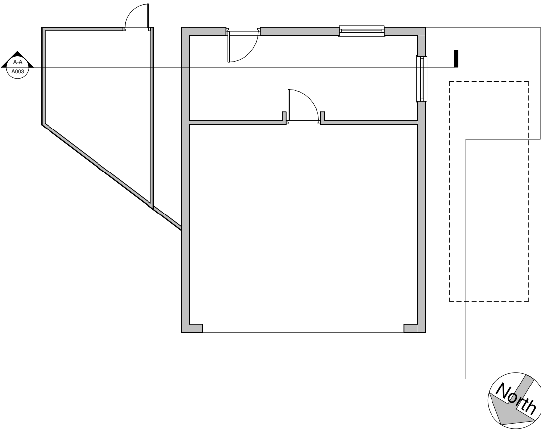
Existing Ground Floor Plan 1 : 50
