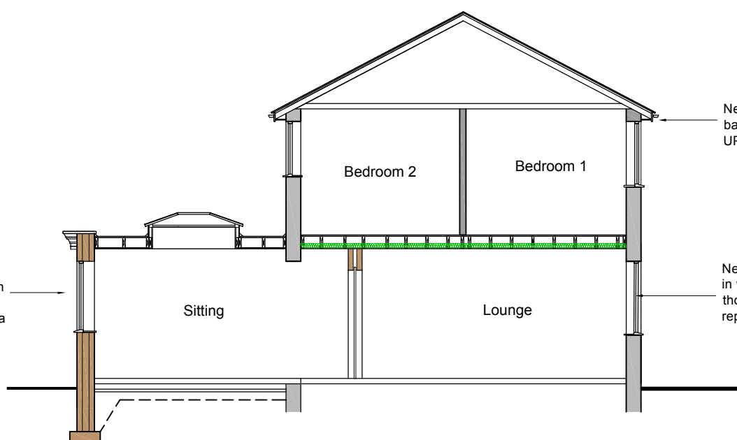
Proposed Section - D - D
