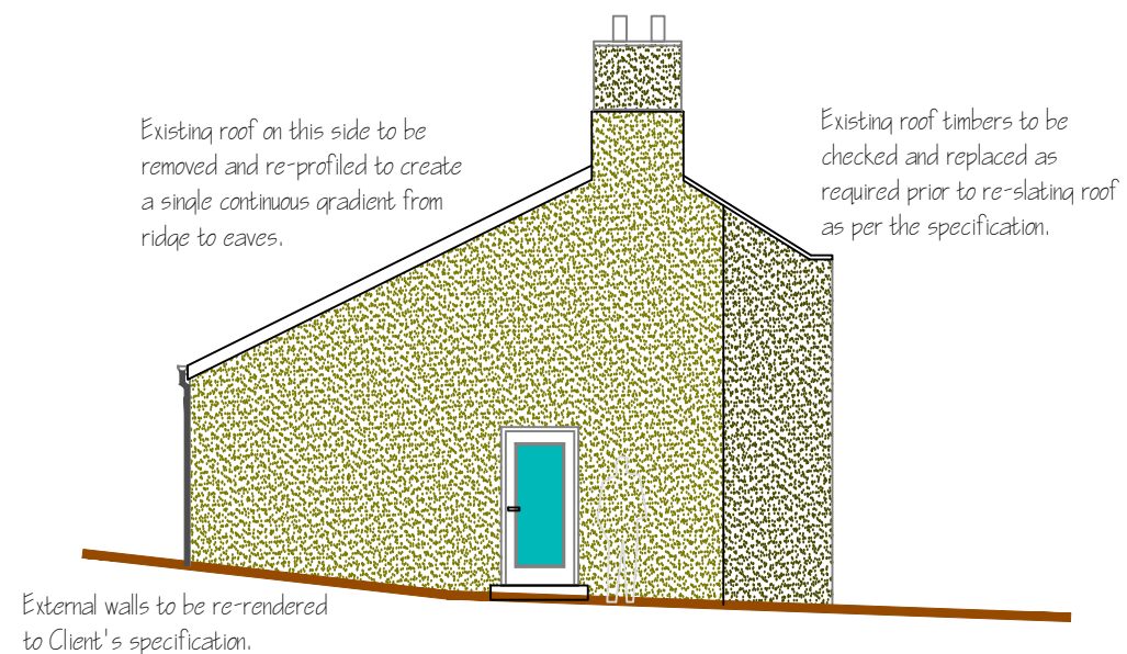
PROPOSED GABLE 2 ELEVATION SCALE 1:100
