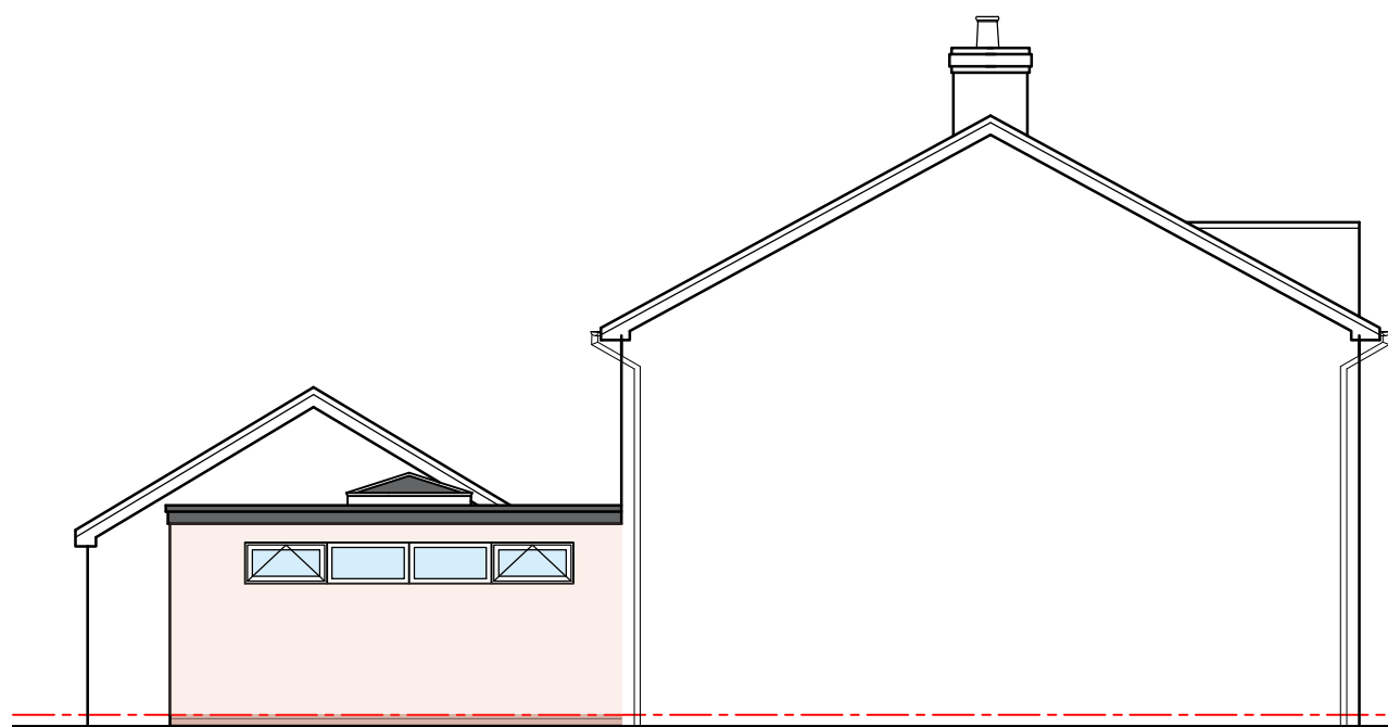
Side elevation 02
