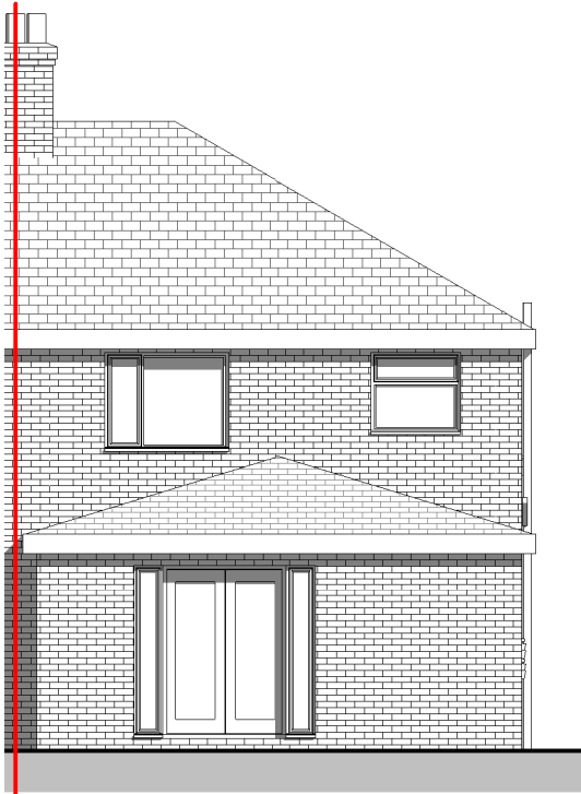
Rear Elevation 1 : 100
