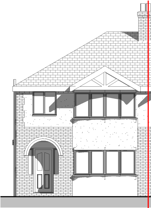
Front Elevation 1 : 100
