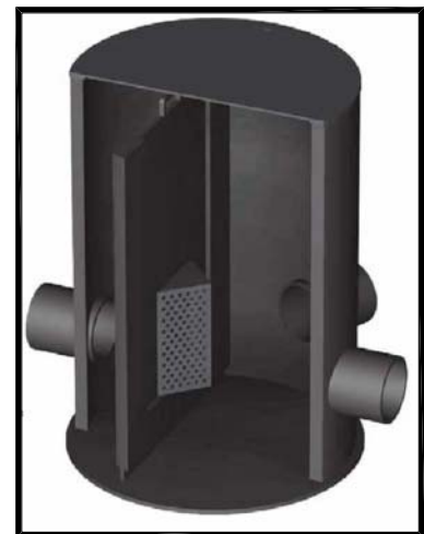
Flow Control
