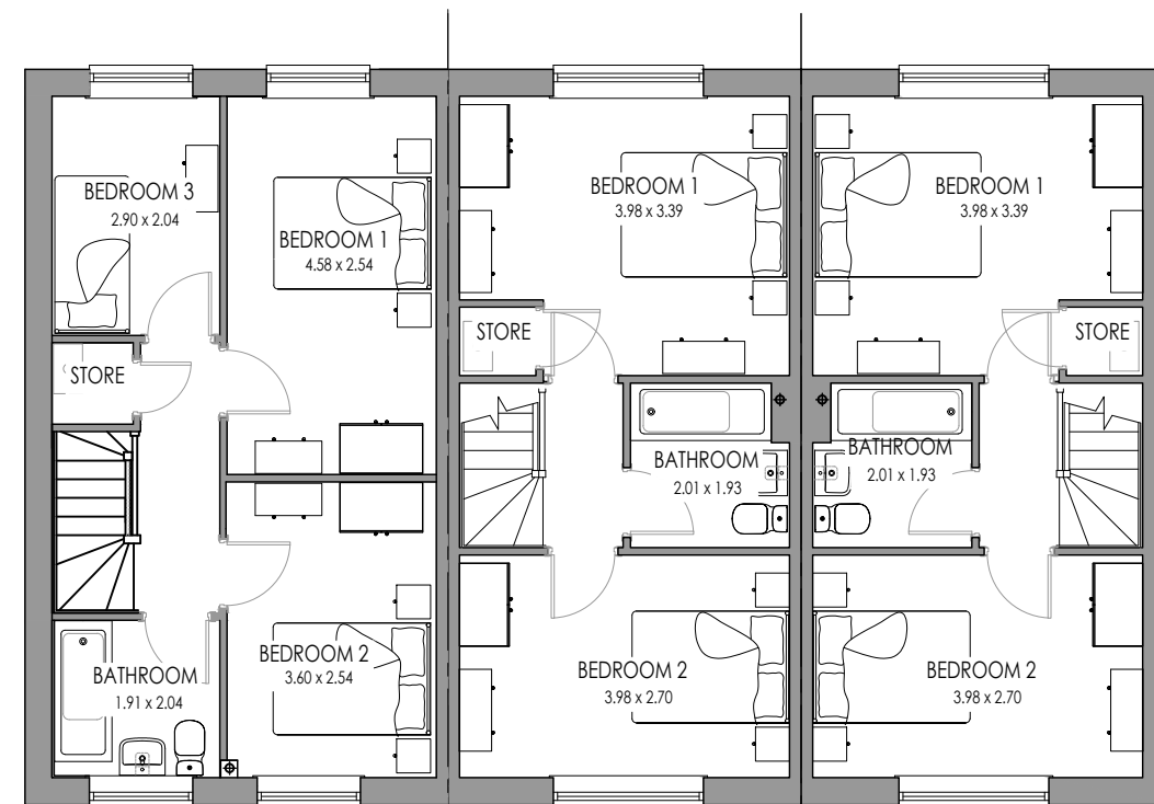
ELWY AS FIRST FLOOR
