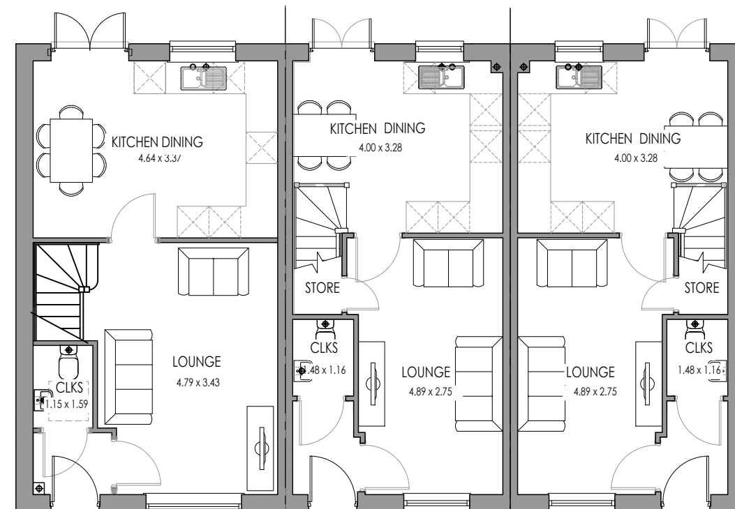
ELWY AS GROUND FLOOR
