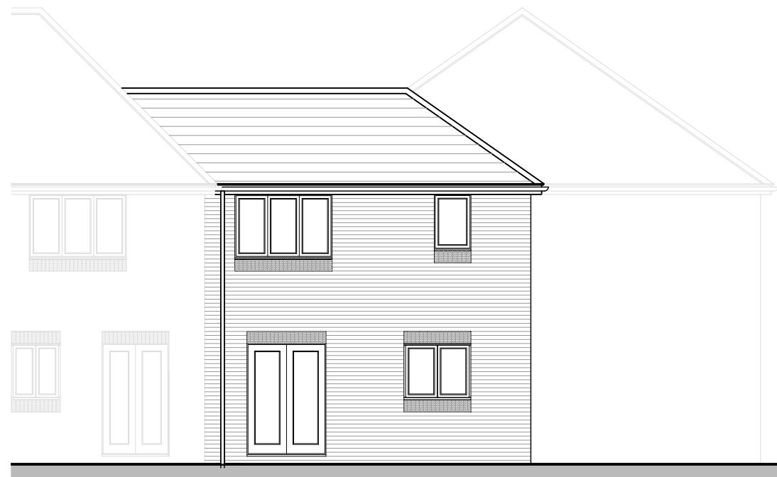
BRONTE AS SIDE ELEVATION
