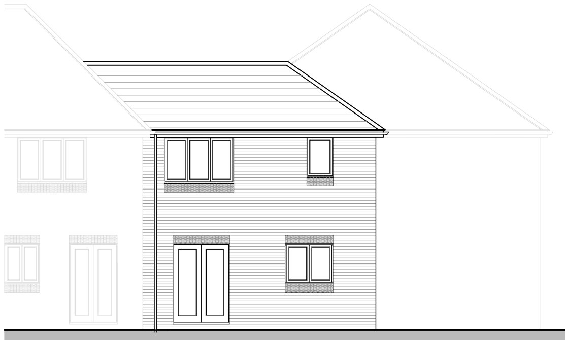
BRONTE AS SIDE ELEVATION
