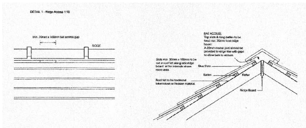
Figure 2: Ridge tile detail.
