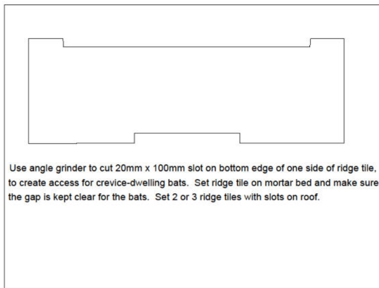
Figure 1: Gaps under ridge tiles.
