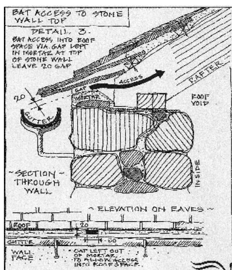
Figure 3: Gaps in eaves detail.
