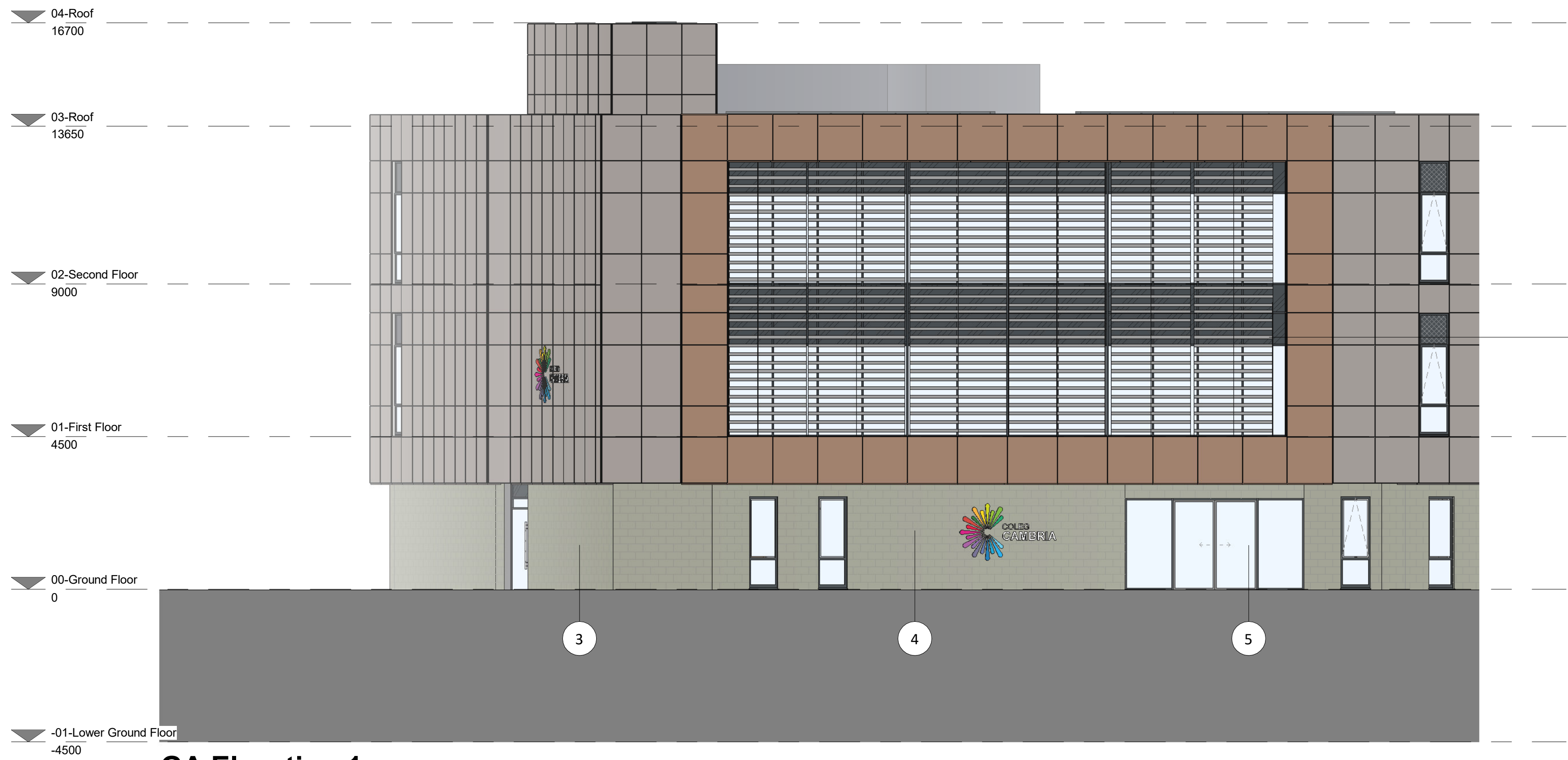
1 GA Elevation 1 1 : 100
