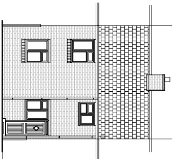
EXISTING REAR ELEVATION (2m to chimney caddy)
