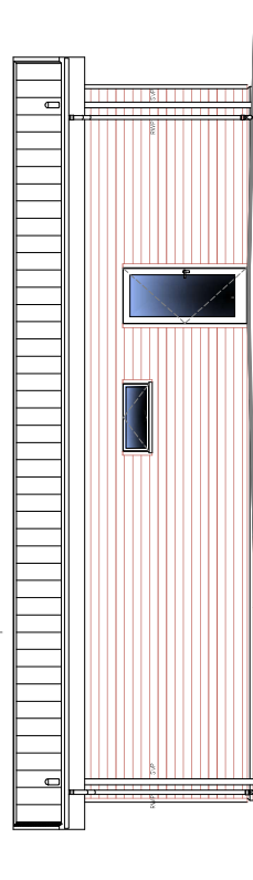
EAST ELEVATION
