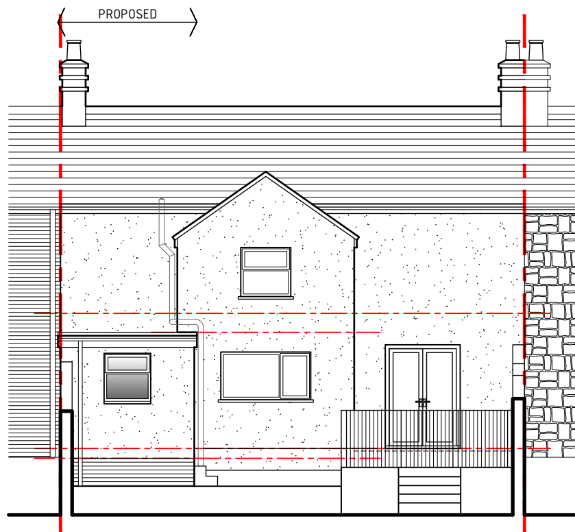
Rear Elevation 1:100
