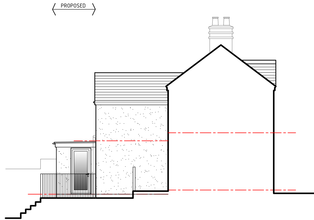
Side-01 Elevation 1:100
