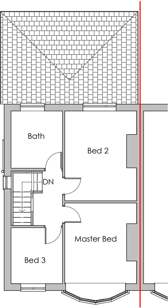
First Floor 1 : 100
