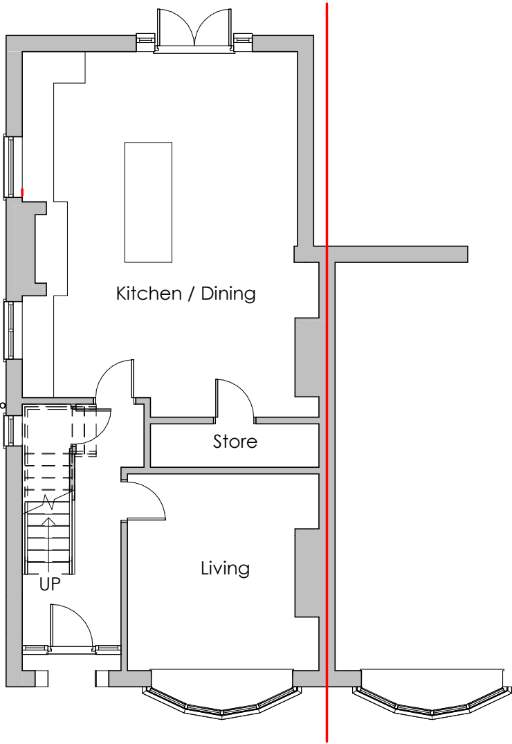
Ground Floor 1 : 100
