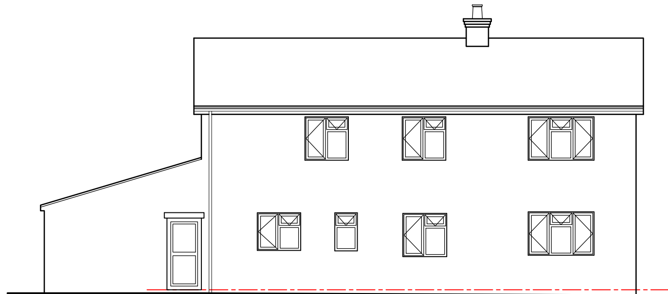
Rear Elevation
