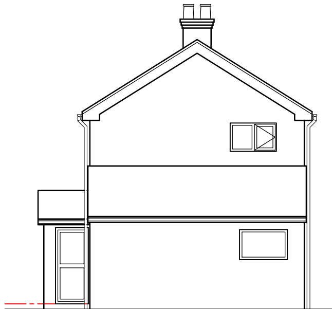
Side 02 Elevation
