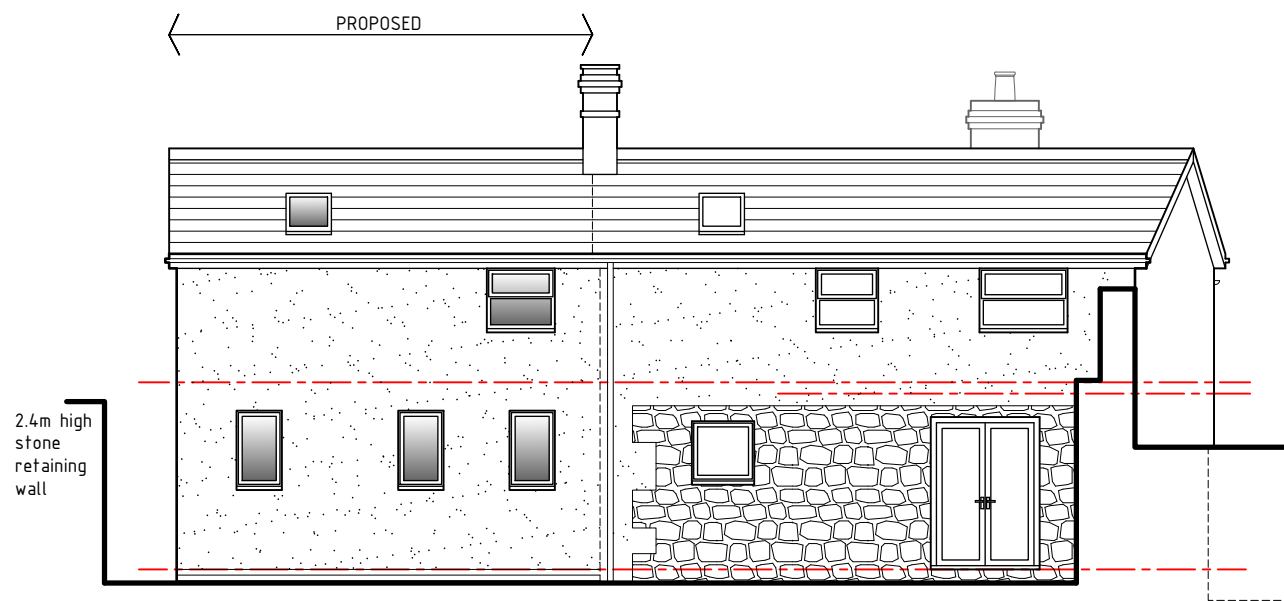
Rear elevation 1:100
