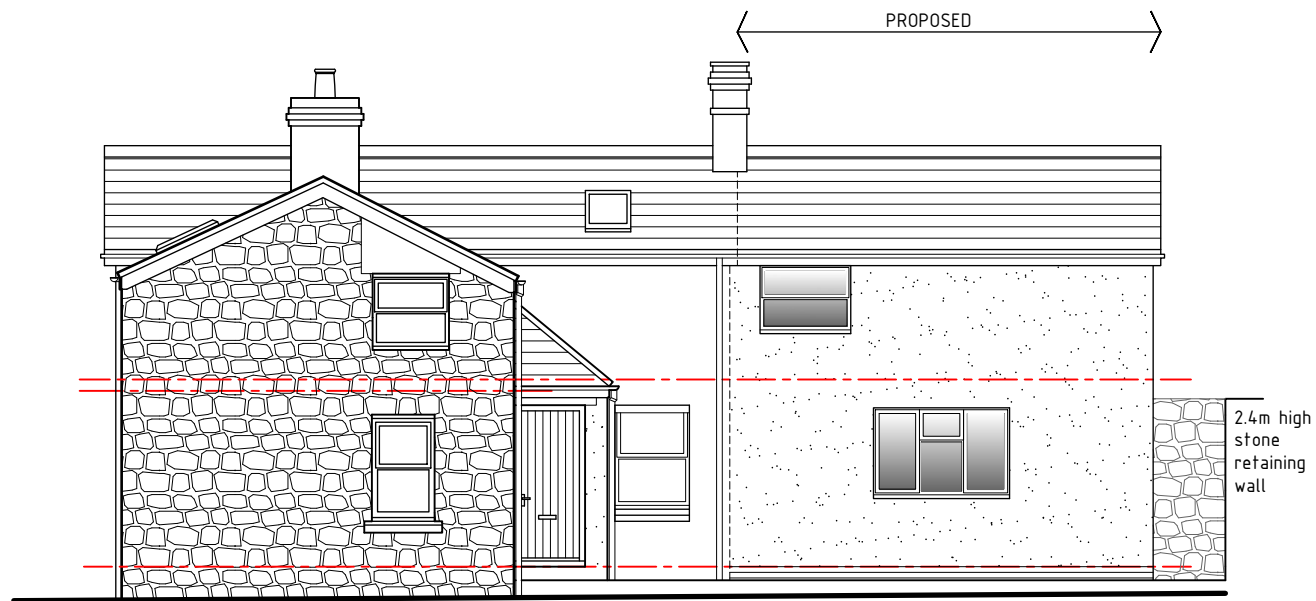
Front elevation 1:100
