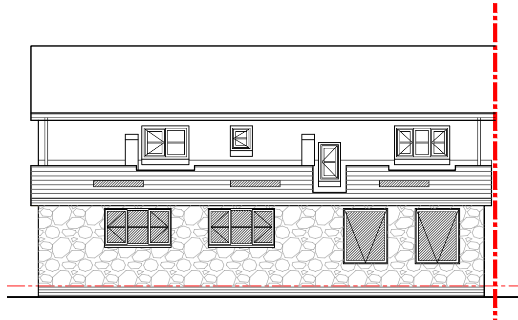
Rear Elevation
