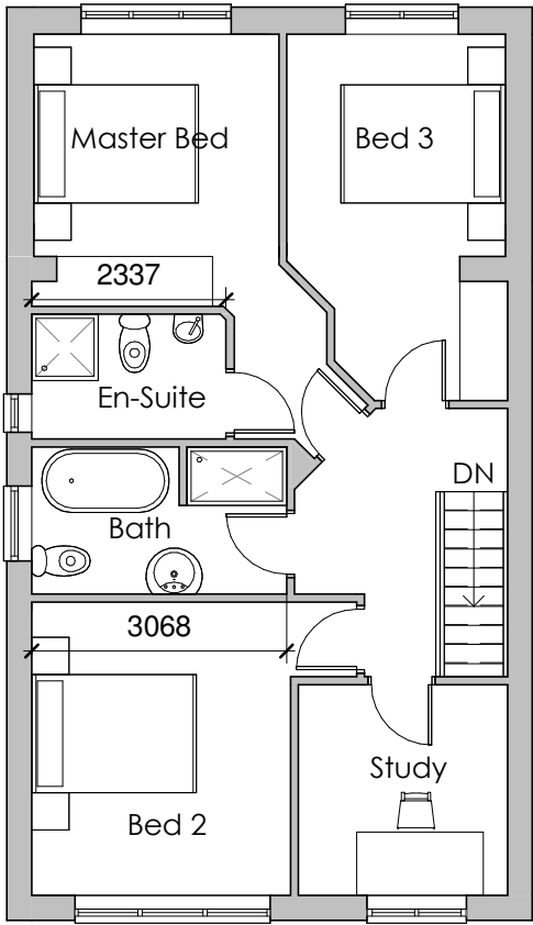
First Floor 1 : 100
