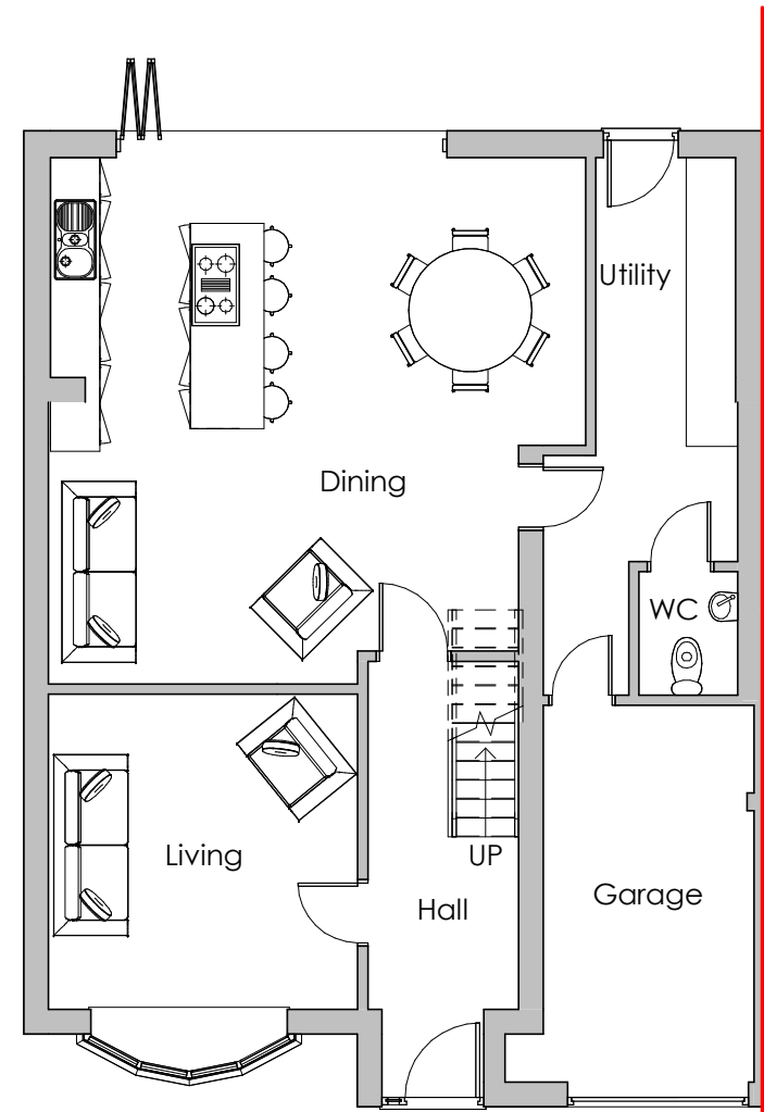
Ground Floor 1 : 100
