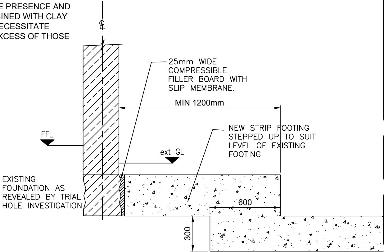
INTERFACE OF NEW TO EXISTING FOUNDATIONS
