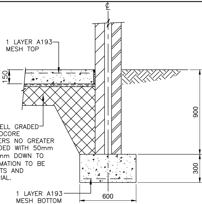
SECTION THROUGH REAR WALL
