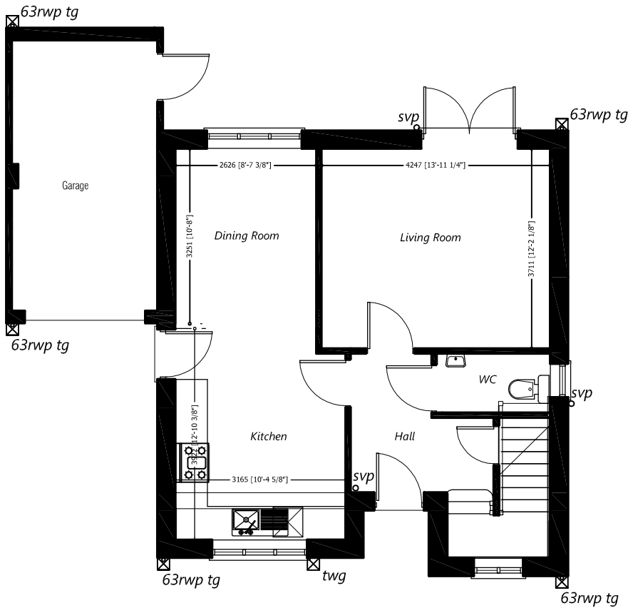
Ground floor layout plan Floor area excl garage: 49.5 q m/532 sq ft
