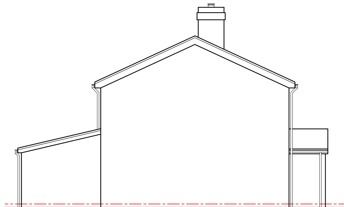
Side 01 Elevation
