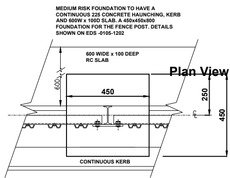
FOUNDATION PLAN
