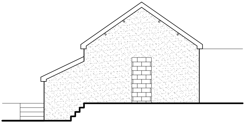
REAR ELEVATION
