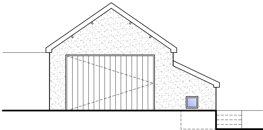
FRONT ELEVATION
