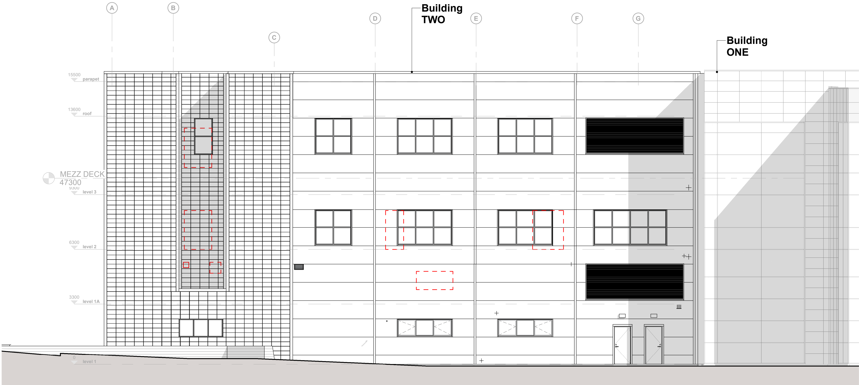
Se Planning_Elevation_GA_South, Existing Scale: 1 : 100
