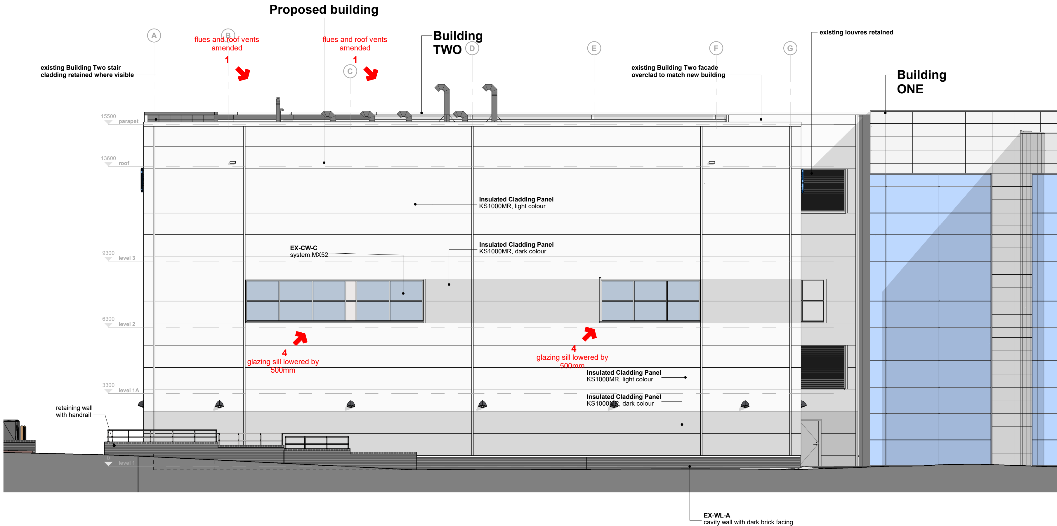
S Planning_Elevation_GA_South Scale: 1 : 100
